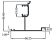
Flying Mullion
