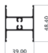
Mesh Mullion
