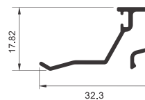
Laminated Glass Bead
