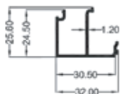
Bead SGU
