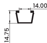
Glass Reducer
