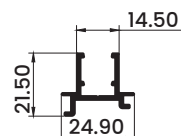
Mating Profile
