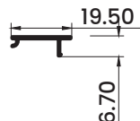
Mesh Adaptor Cap
