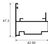
Flying Mullion
