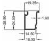
Bead DGU
