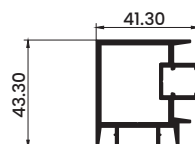
Corner Profile
