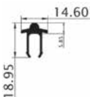
Guide Rail
