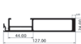
Sash Reinforced Interlock
