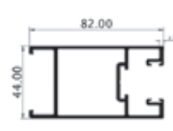
Sash Handle 82
