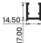
Add-on Track
